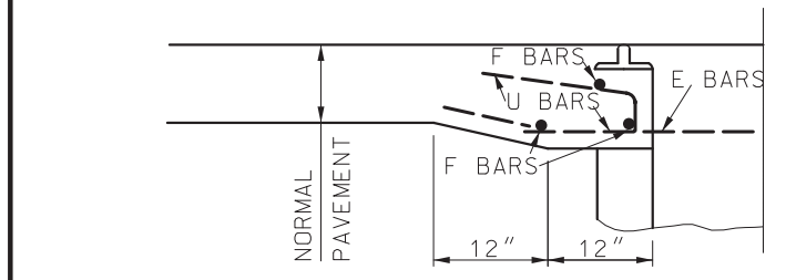
HALF SECTION F-F
