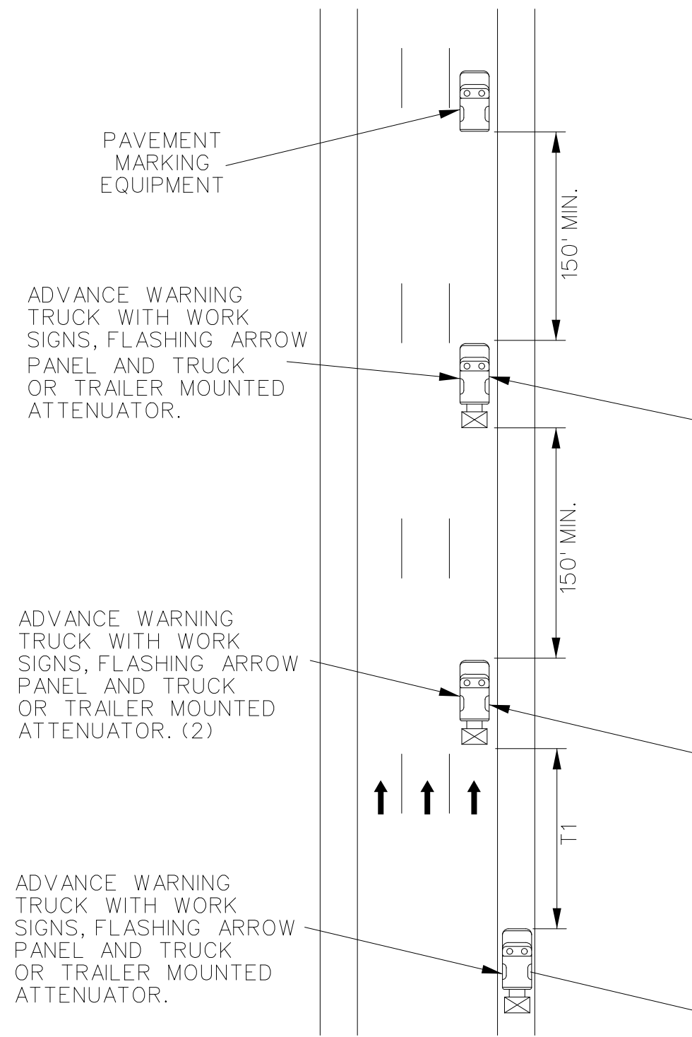
MULTI-LANE DIVIDED HIGHWAY MOVING OPERATION ON HIGHWAY OPEN TO TRAFFIC
