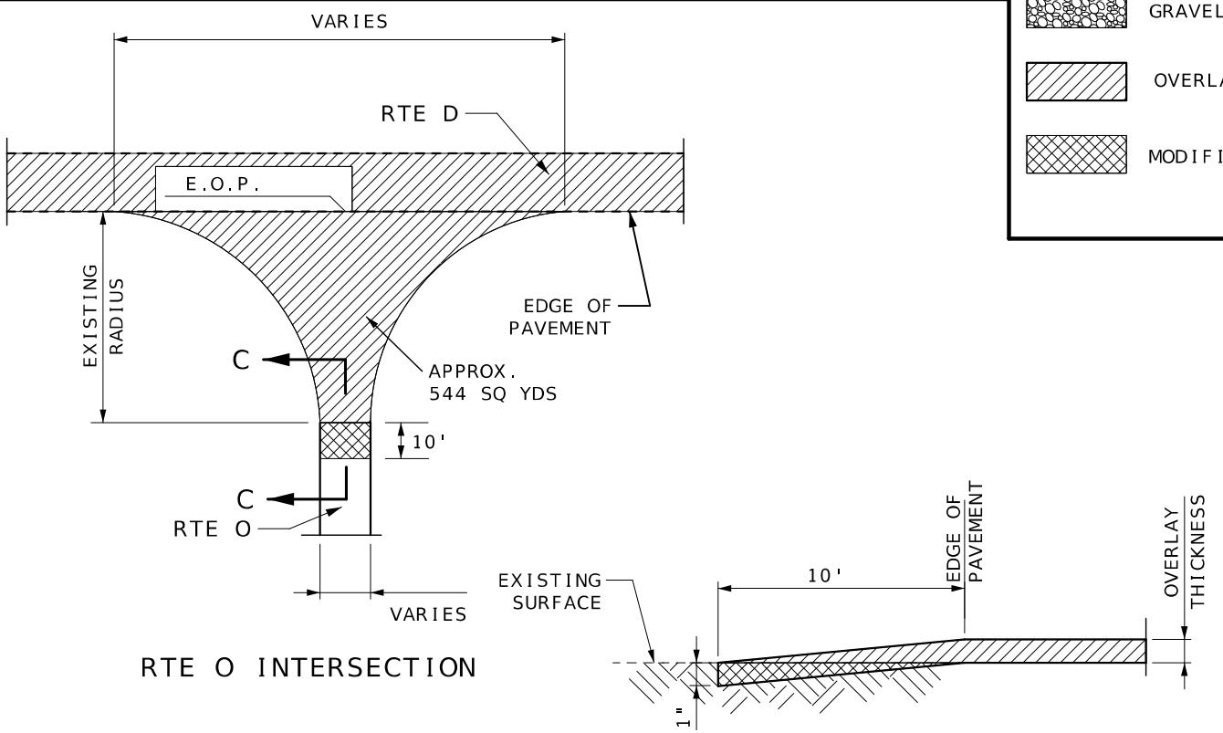
SECTION C-C INTERSECTION OF ROUTE O
