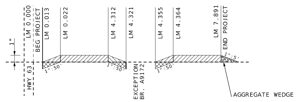
LONGITUDINAL TRAVELWAY DEPTH TRANSITION
