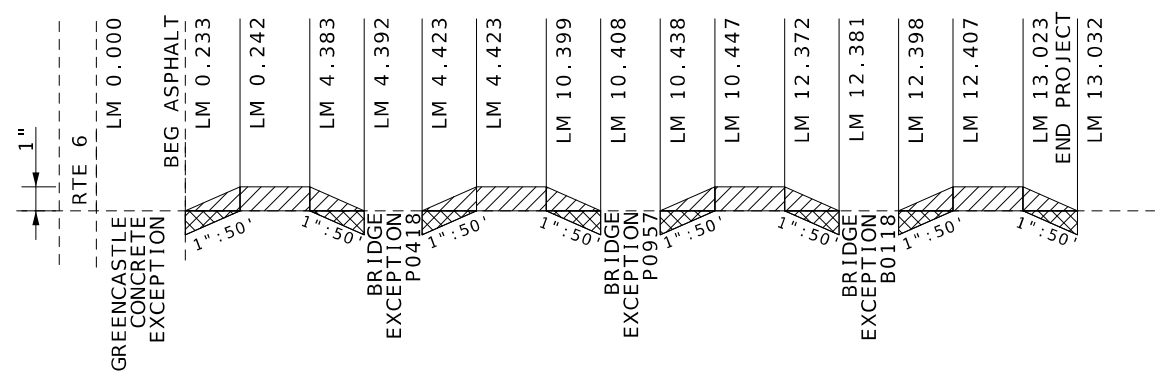
LONGITUDINAL TRAVELWAY DEPTH TRANSITION
