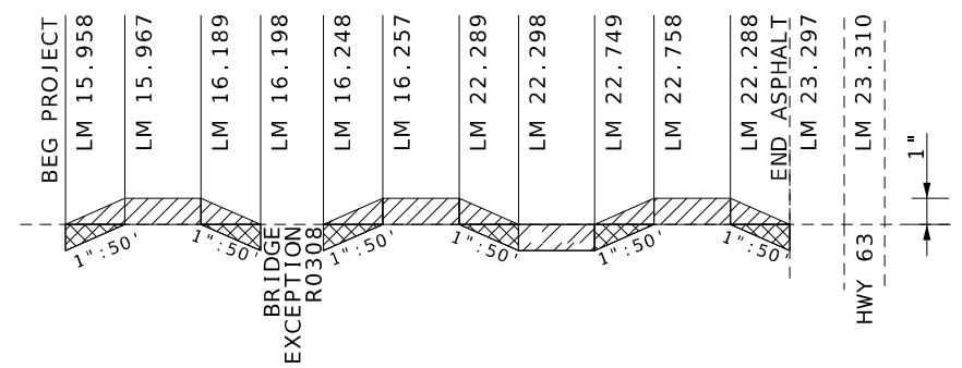
LONGITUDINAL TRAVELWAY DEPTH TRANSITION
