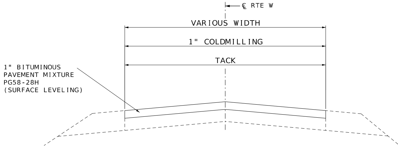
TYPICAL SECTION
