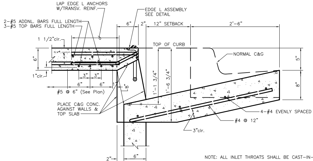
THROAT DETAIL
