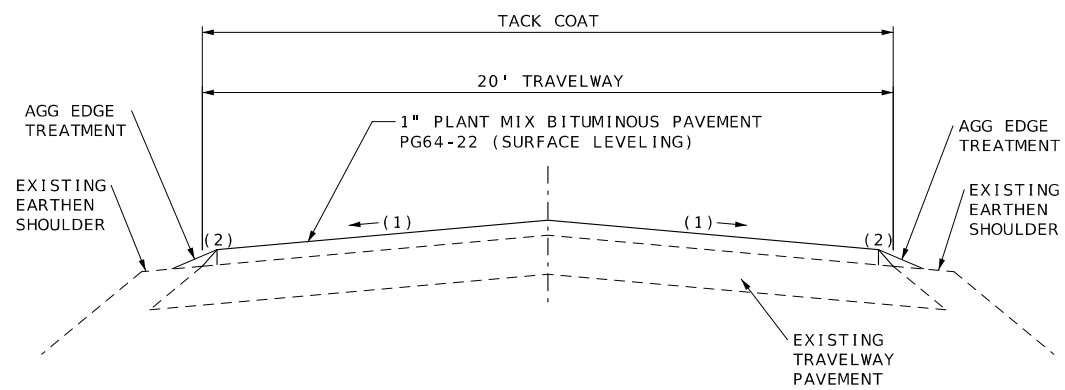
TYPICAL SECTION ROUTE 95 LOG MILE 42.007 - 51.467
