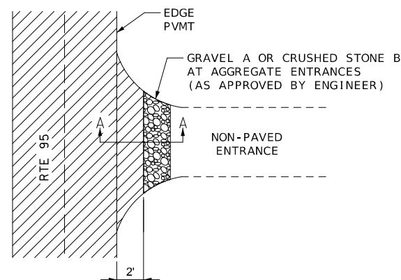
PLAN VIEW FOR NON-PAVED PRIVATE AND COMMERCIAL ENTRANCES WITH EXISTING APRON
