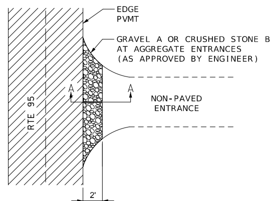
PLAN VIEW FOR NON-PAVED PRIVATE AND COMMERCIAL ENTRANCES WITHOUT EXISTING APRON
