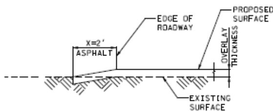
SECTION B-B TYPICAL ASPHALT ENTRANCE
