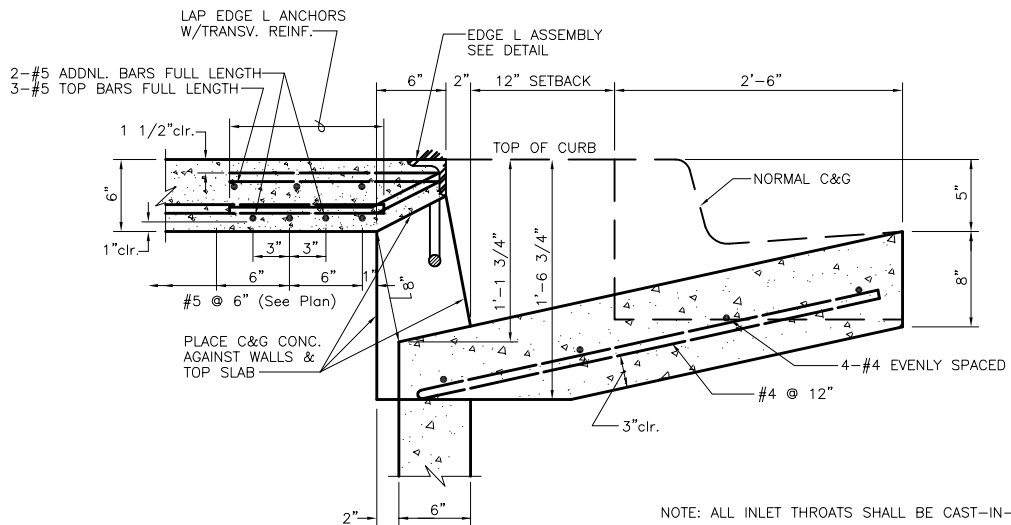
THROAT DETAIL
