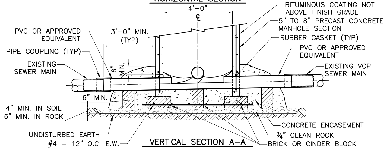
HORIZONTAL SECTION
