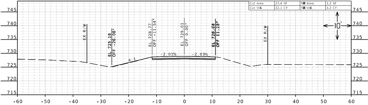
STA 462+75.00 R2 END PROJECT J3S3178
