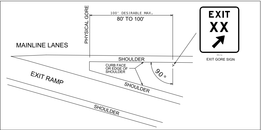
EXIT GORE SIGN LOCATION DETAIL
