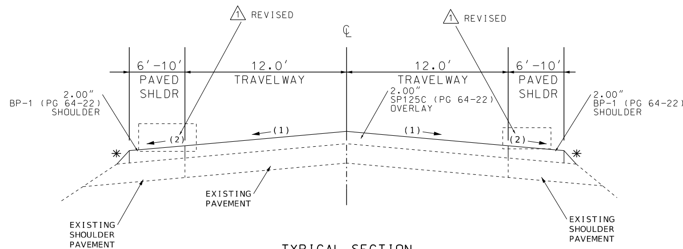
TYPICAL SECTION MO 5
