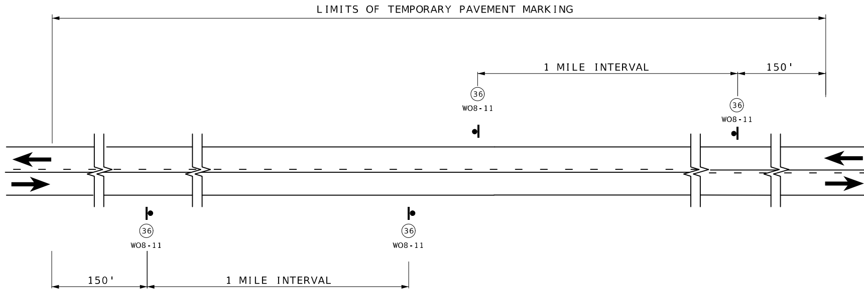
SIGN SPACING AND TEMPORARY STRIPING FOR MAINLINE
