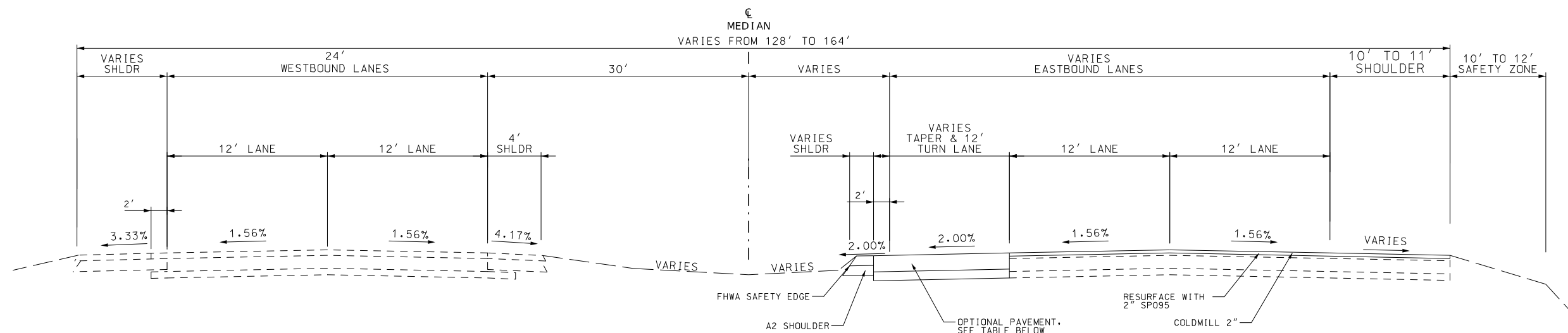
PROPOSED TYPICAL SECTION ROUTE 36 (EBL AND WBL) STA. 1155+60.00 TO STA. 1157+60.00
