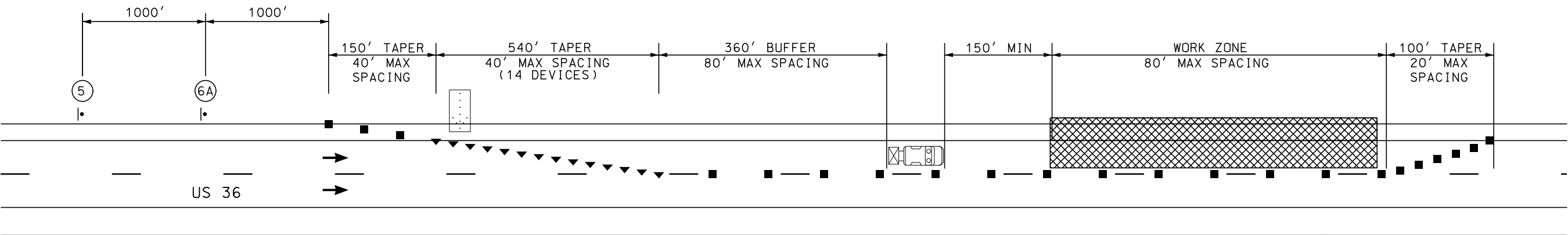
LEFT LANE CLOSURE NOT TO SCALE
