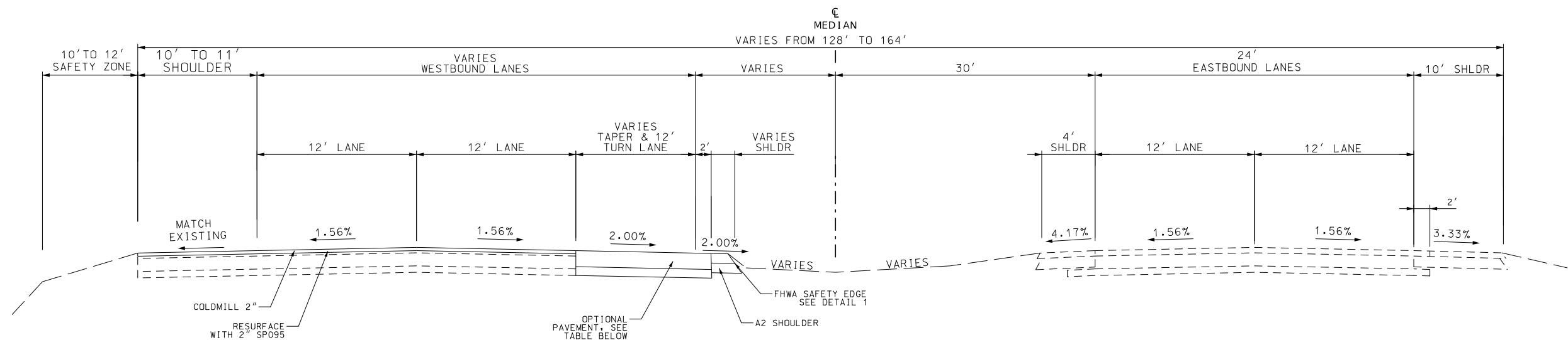
PROPOSED TYPICAL SECTION ROUTE 36 (EBL AND WBL) STA. 1166+65.00 TO STA. 1168+62.00
