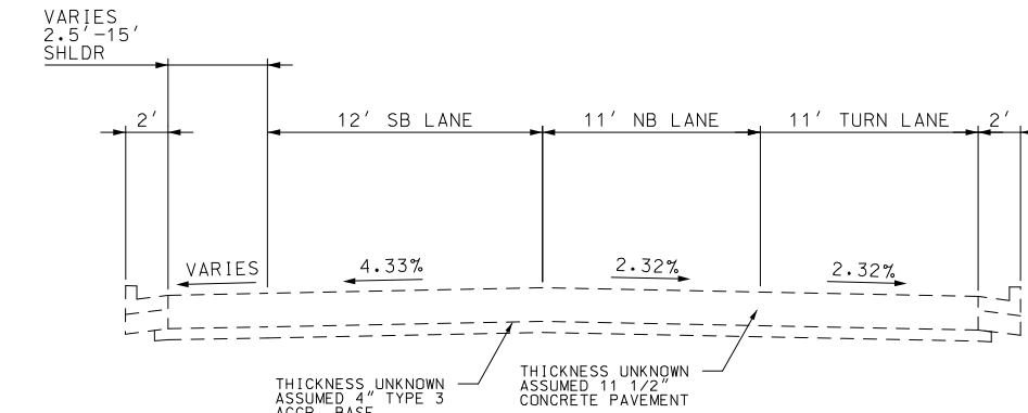
EXISTING TYPICAL SECTION BOB F. GRIFFIN RD (SOUTH OF RTE 36) STA. 8+04.39 TO STA. 11+47.94
