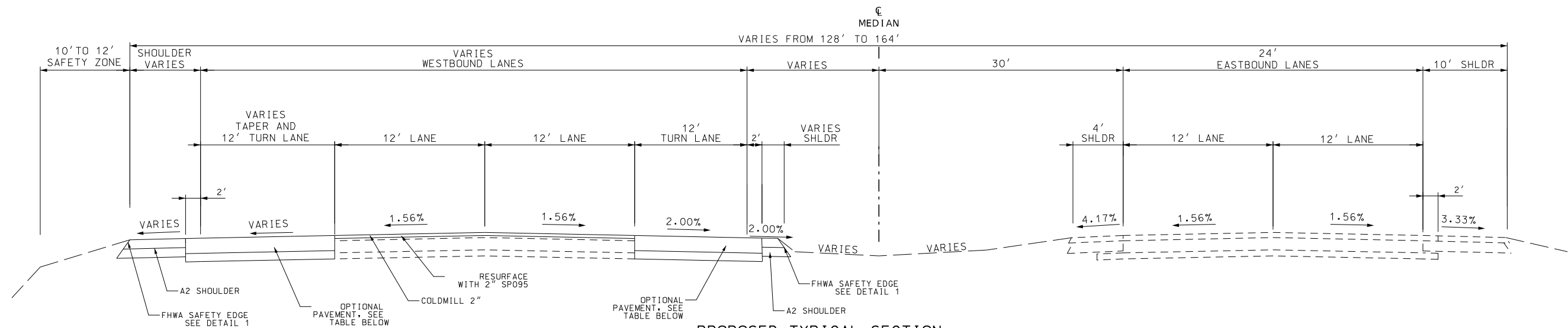
PROPOSED TYPICAL SECTION ROUTE 36 (EBL AND WBL) STA. 1163+85.00 TO STA. 1166+65.00
