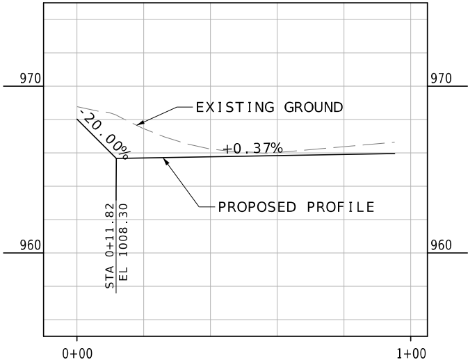
SOUTHEAST DITCH  US 36 STA 1162+91.28 TO STA 1163+85.00
