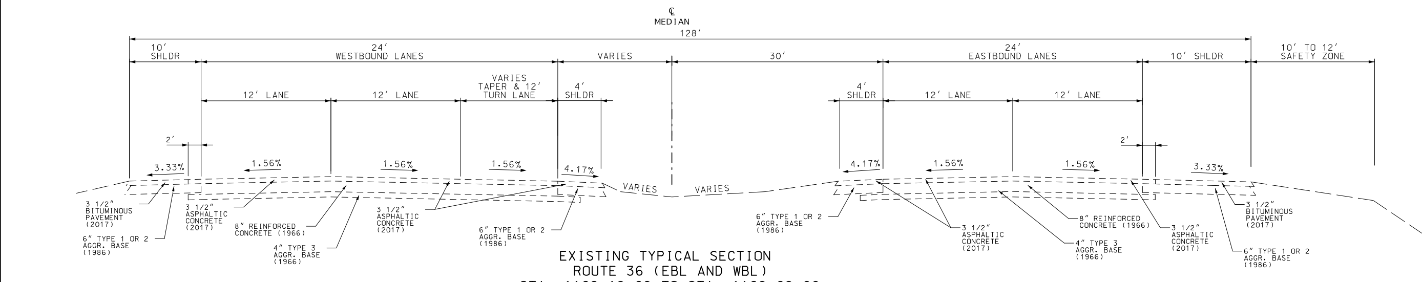
EXISTING TYPICAL SECTION ROUTE 36 (EBL AND WBL) STA. 1155+63.44 TO STA. 1161+96.80
