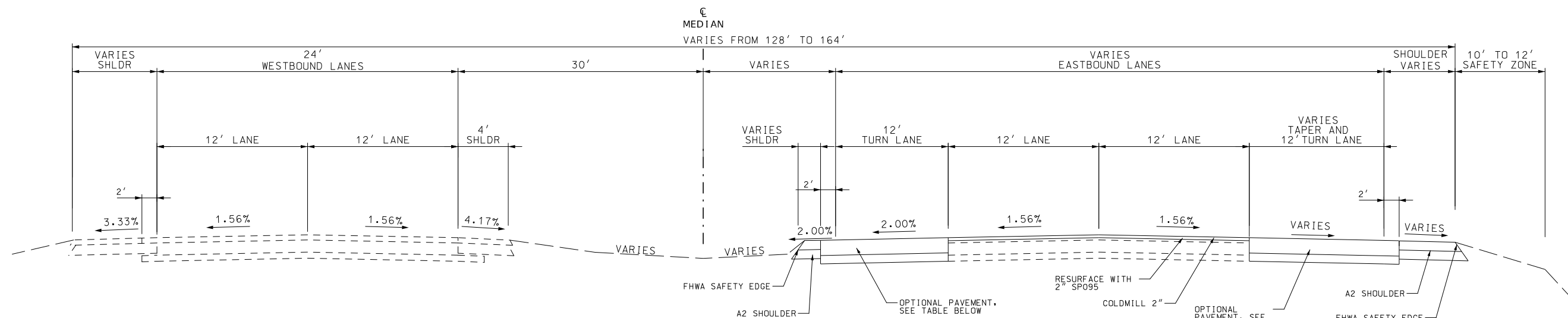
PROPOSED TYPICAL SECTION ROUTE 36 (EBL AND WBL) STA. 1157+60.00 TO STA. 1160+35.00
