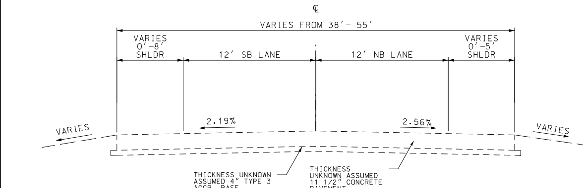
EXISTING TYPICAL SECTION BOB F. GRIFFIN RD (NORTH OF RTE 36) STA. 33+56.63 TO STA. 37+12.59
