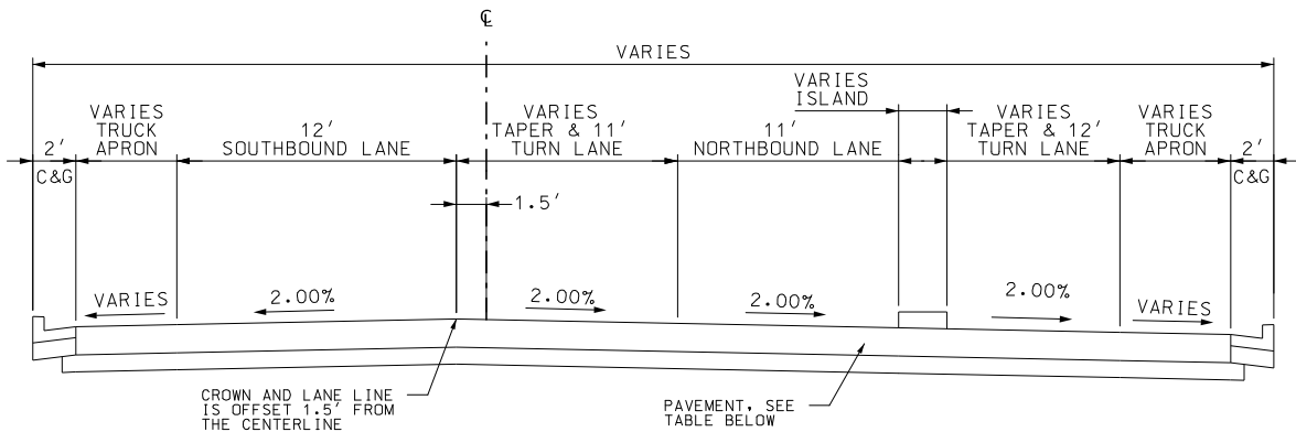
PROPOSED TYPICAL SECTION BOB F. GRIFFIN RD (NORTH OF RTE 36) STA. 33+56.66 TO STA. 37+12.59
