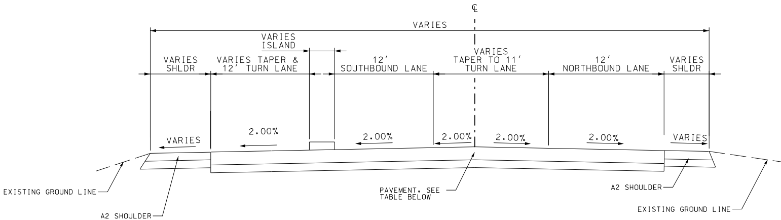
PROPOSED TYPICAL SECTION BOB F. GRIFFIN RD (NORTH OF RTE 36) STA. 33+56.66 TO STA. 37+12.59
