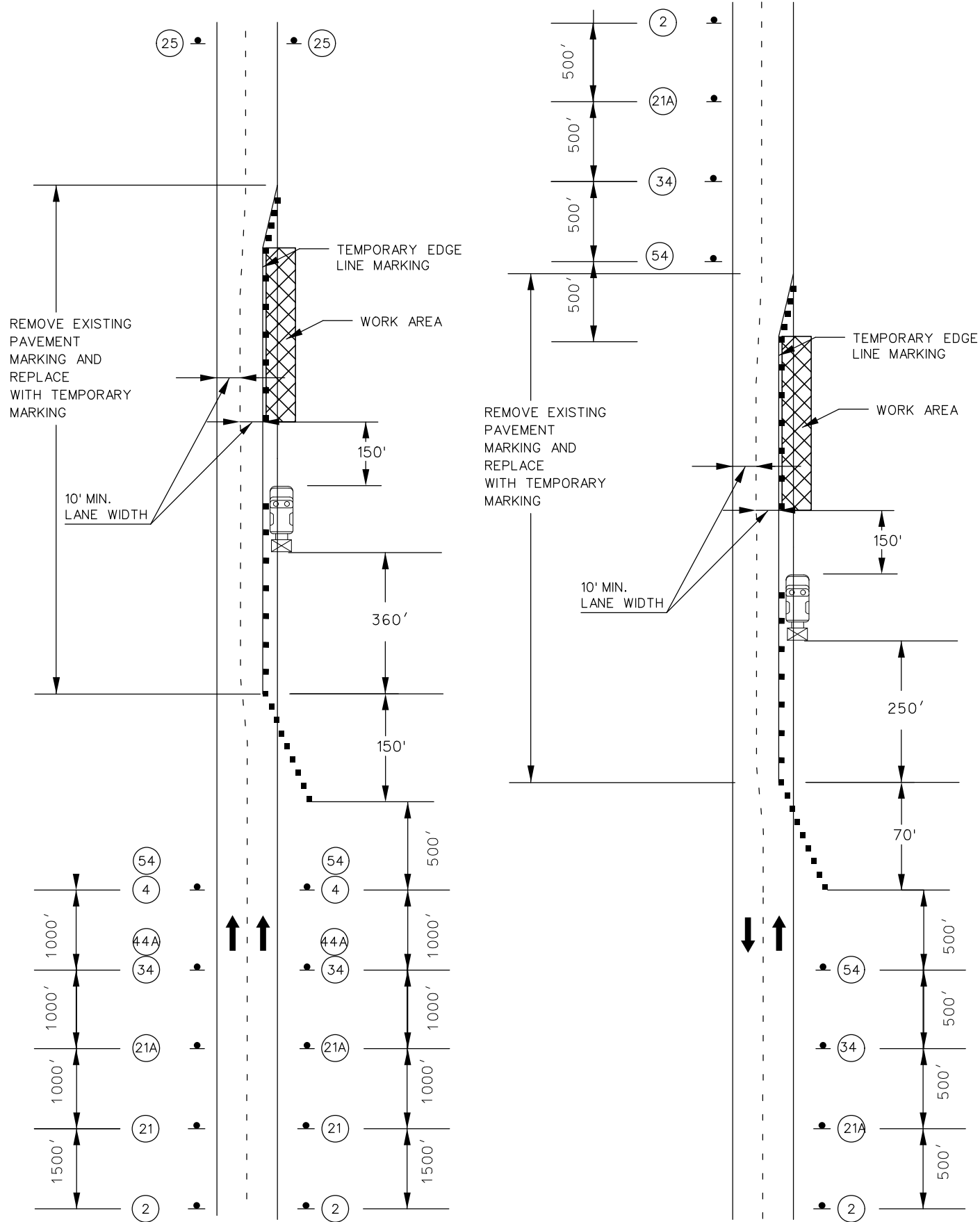
SHOULDER WORK ON DIVIDED HIGHWAY REDUCED LANE WIDTHS
