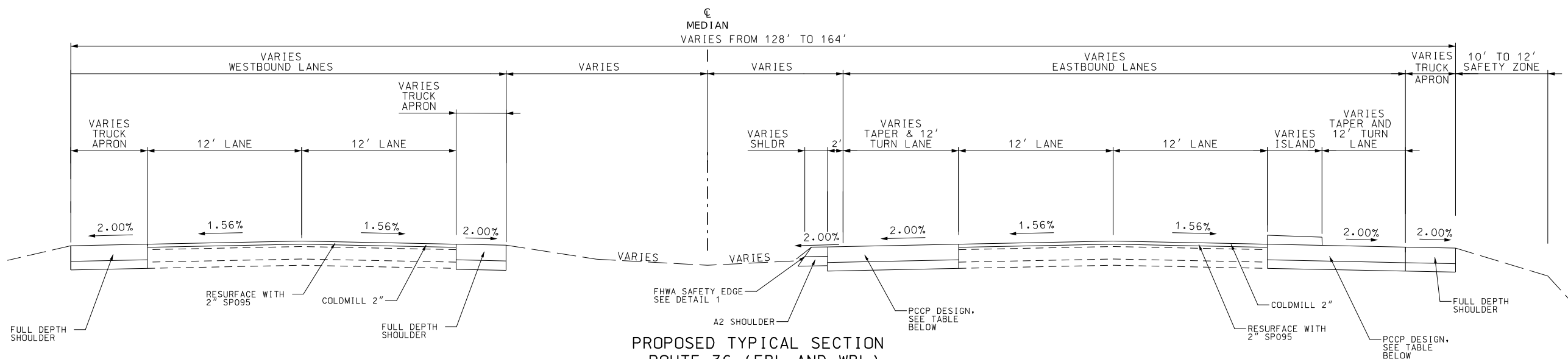
PROPOSED TYPICAL SECTION ROUTE 36 (EBL AND WBL) STA. 1160+35.00 TO STA. 1161+27.73
