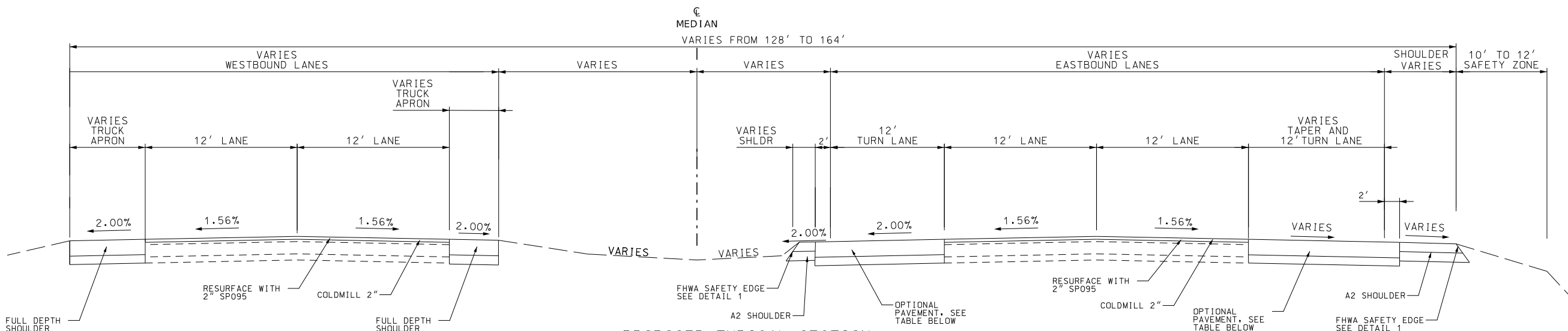
PROPOSED TYPICAL SECTION ROUTE 36 (EBL AND WBL) STA. 1160+35.00 TO STA. 1161+27.73
