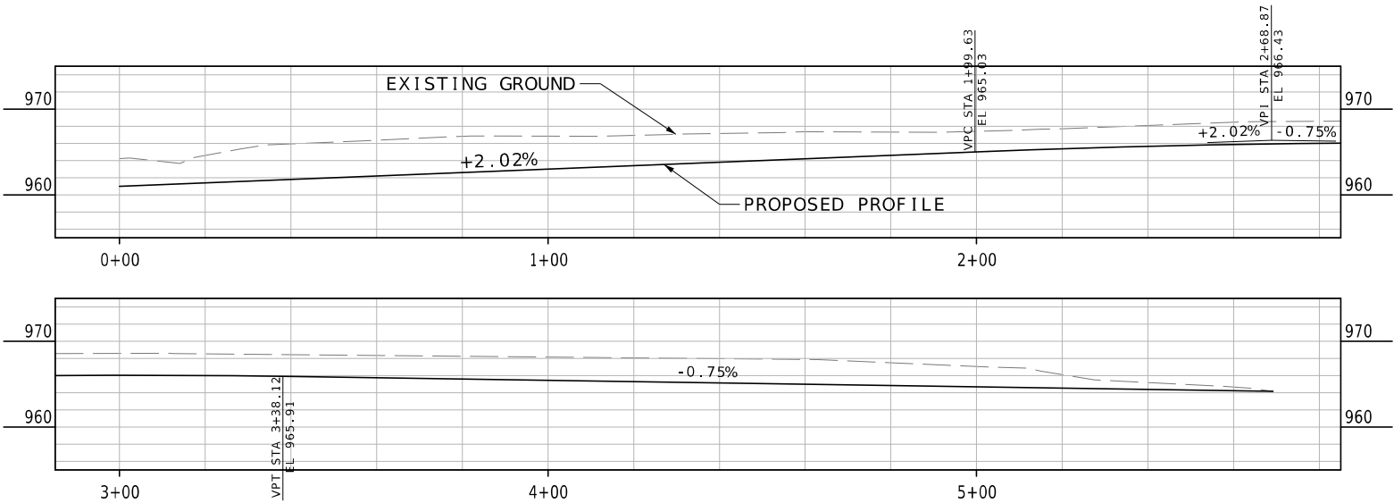
NORTHEAST DITCH  US 36 STA 1162+27.46 TO STA 1167+44.56
