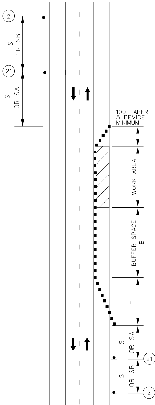
WORK ON THE SHOULDER ON UNDIVIDED HIGHWAYS
