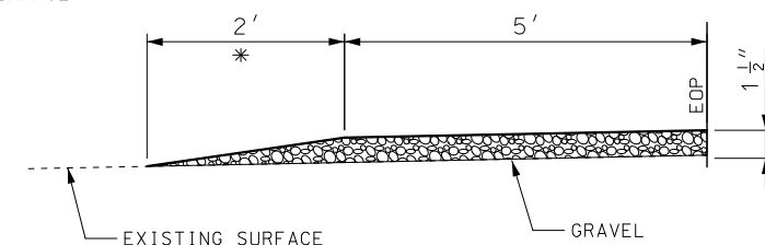
TYPICAL UNPAVED ENTRANCE (FIELD, PRIVATE OR COUNTY ROAD) * TAPER AT 1:1 FOR FIELD ENTRANCE
