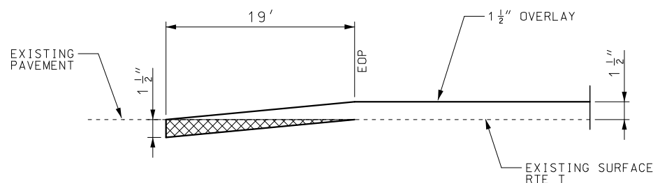
TYPICAL SIDE ROAD (COLDMILLED TRANSITION)
