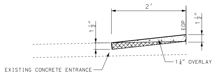
TYPICAL CONCRETE ENTRANCE 2' COLDMILLED TRANSITION
