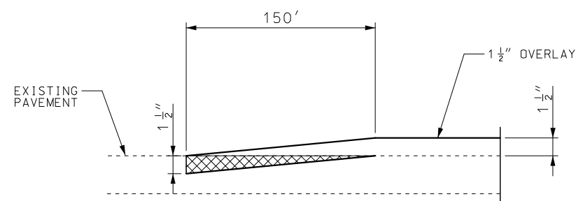
TRAVELWAY DEPTH TRANSITIONS BEGINNING AND END OF PROJECT AND EXCEPTIONS
