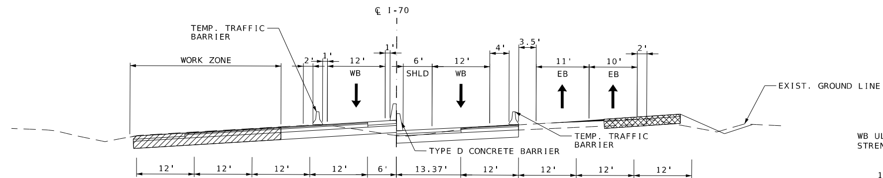
SECTION ON CURVE TYPICAL SECTION I-70 PHASE 2
