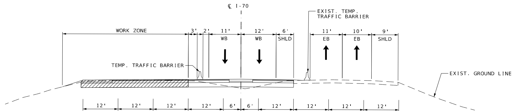
SECTION ON TANGENT TYPICAL SECTION I-70 PHASE 2
