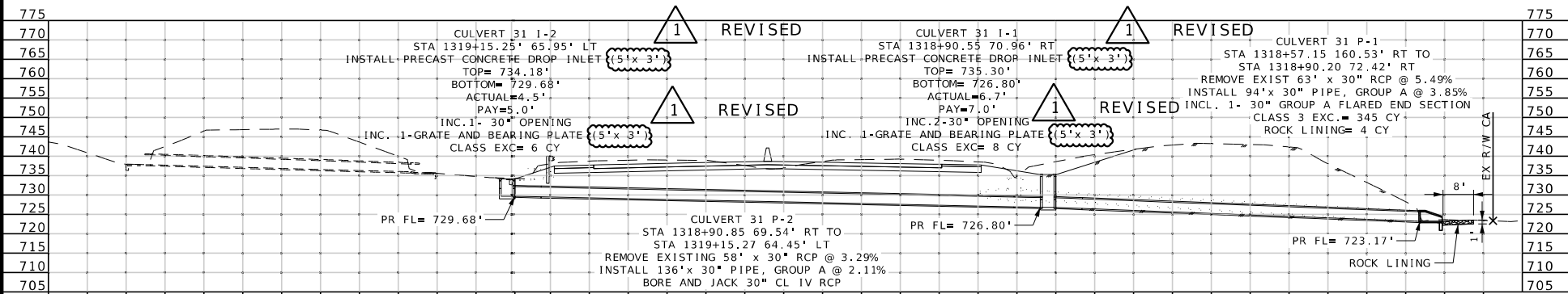
CULVERT 31 (STA 1319+14.41)
