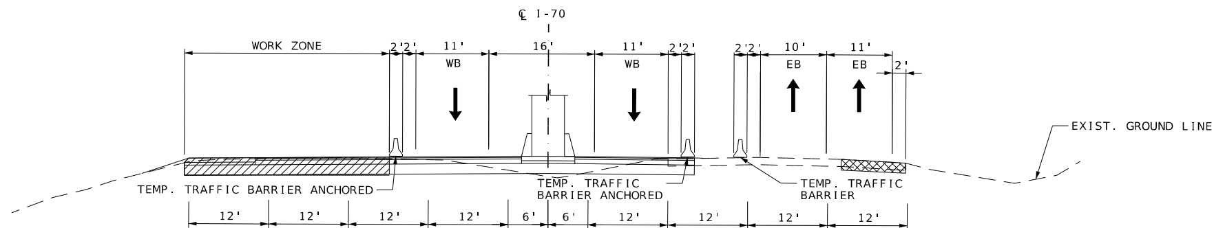
SECTION ON CURVE TYPICAL SECTION I-70 PHASE 2
