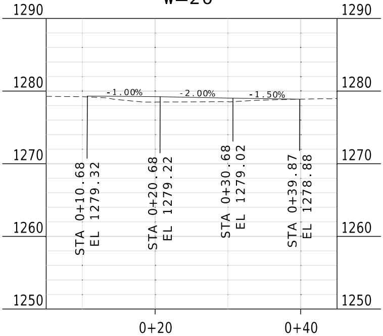
ENTRANCE 8 PROFILE - TYPE 1 DRIVEWAY 3+39.66 RTE_B_CL 10.7' RT W=20'
