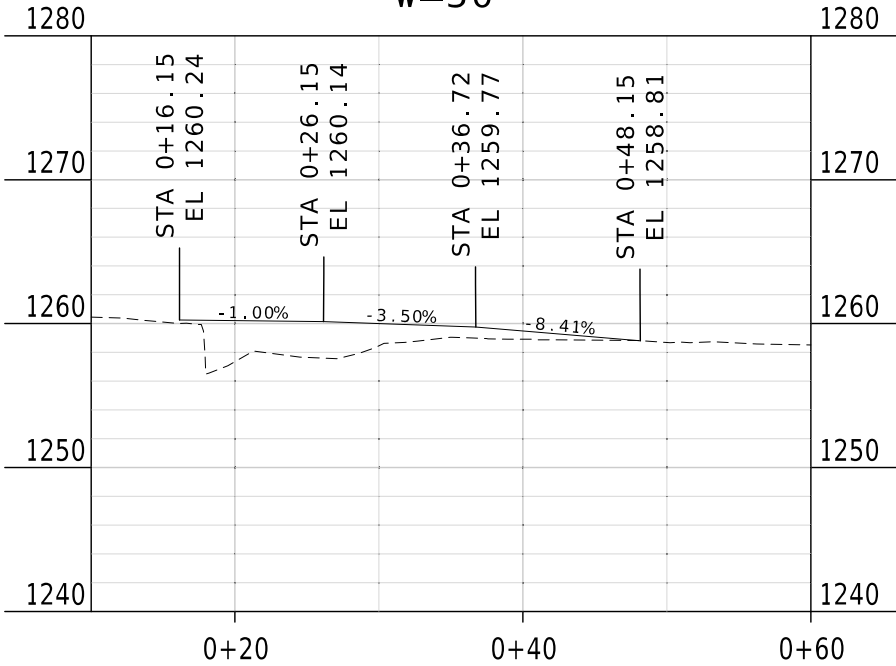
ENTRANCE 2 PROFILE - TYPE 1 DRIVEWAY 532+10.32, RTE 266 16.1' RT W=30'
