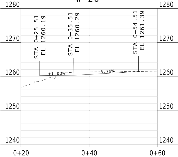
ENTRANCE 1 PROFILE - TYPE 1 DRIVEWAY 532+10.16, RTE 266 25.5' LT W=20'
