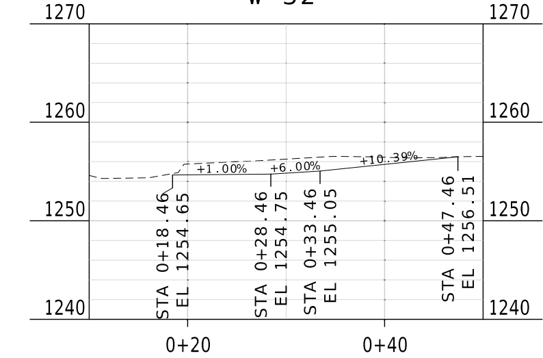
ENTRANCE 5 PROFILE - TYPE 1 DRIVEWAY 4+64.39, FR 99 18.5' LT W=32'
