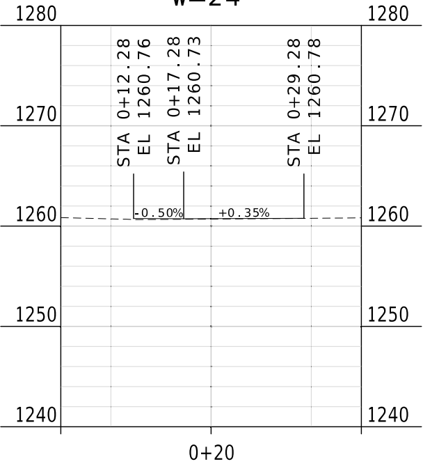
ENTRANCE 3 PROFILE - TYPE 1 DRIVEWAY 351+15.92, RTE AB 12.3' LT W=24'
