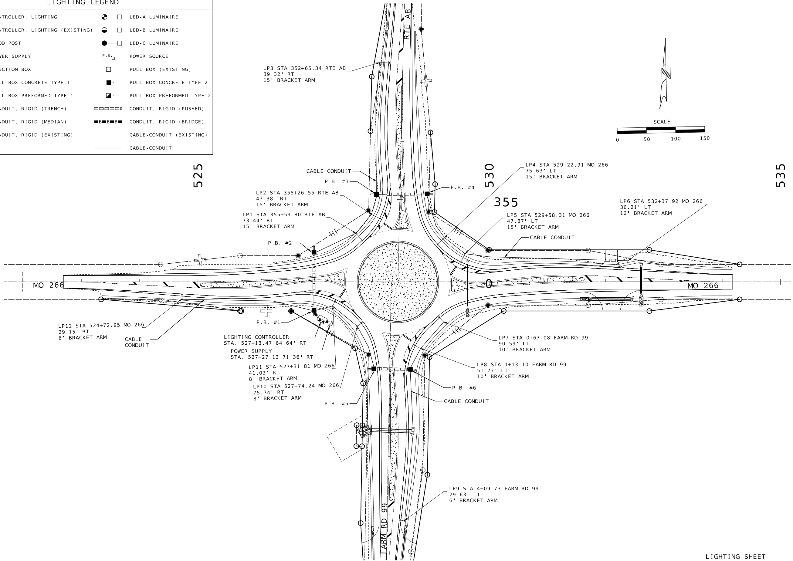
LIGHTING SHEET SHEET 1 OF 2
