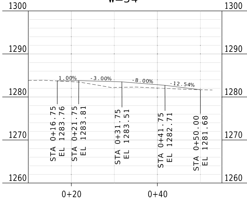
ENTRANCE 7 PROFILE - TYPE 1 DRIVEWAY 559+71.76, RTE 266 16.7' LT W=34'
