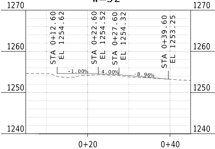
ENTRANCE 4 PROFILE - TYPE 1 DRIVEWAY 4+64.39, FR 99 12.6' RT W=32'
