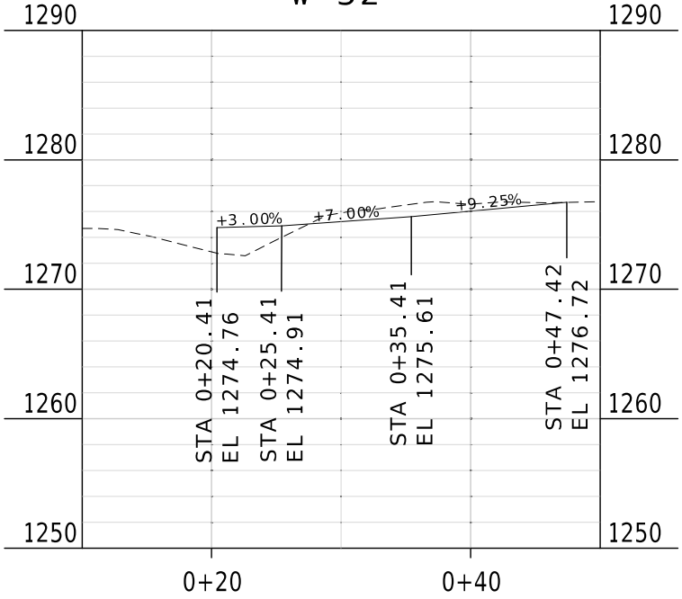
ENTRANCE 6 PROFILE - TYPE 1 DRIVEWAY 550+66.27, RTE 266 20.4' RT W=32'
